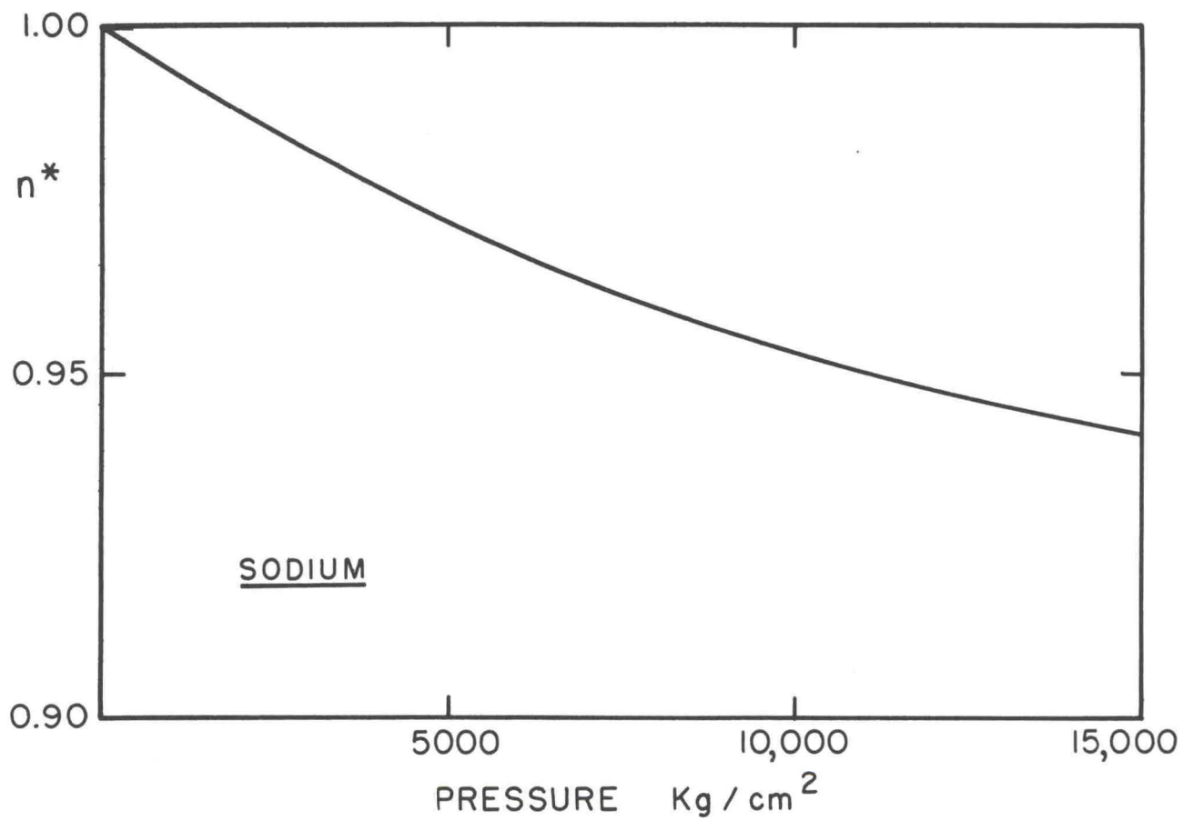
FIG. 3-11 n^* , NORMALIZED ELECTRONS/ATOM VS. PRESSURE
